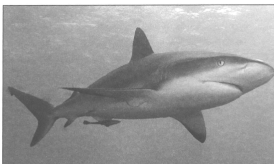
Caribbean reef shark
